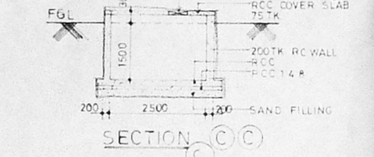
SECTION (C-C)
