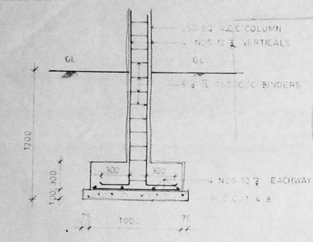
TYPICAL CROSS SECTION OF COLUMN FOOTING
