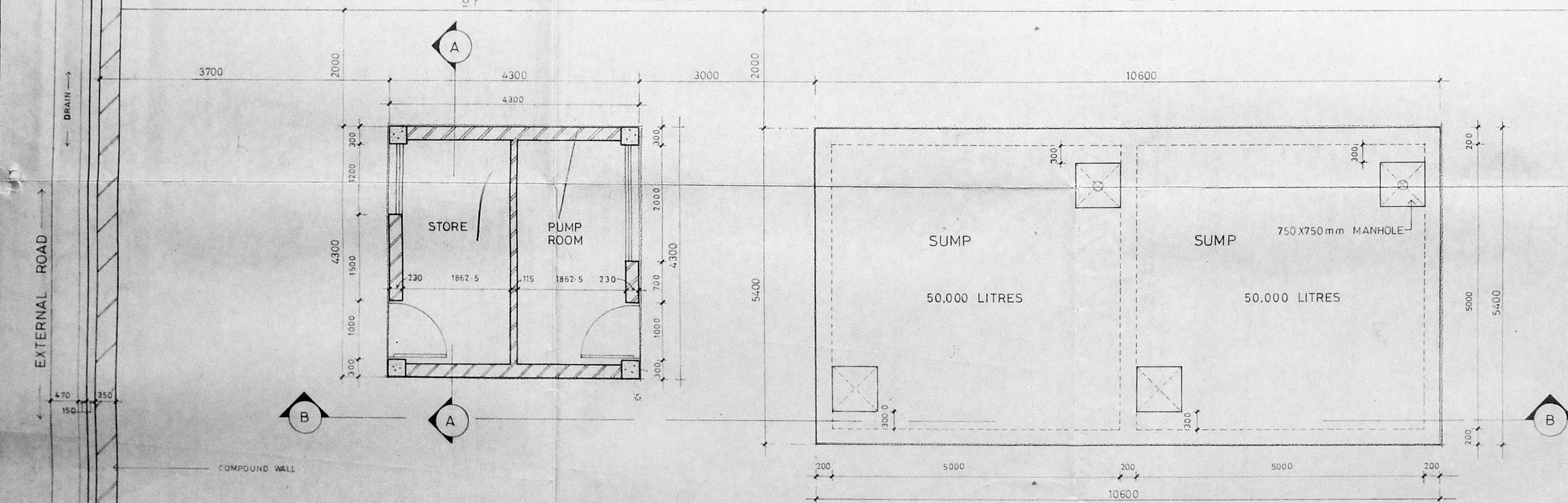
DETAILED SITE PLAN (OHT & SUMP) SCALE 1:50
