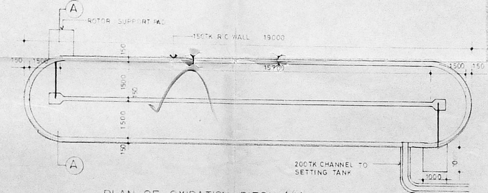
PLAN OF OXIDATION DITCH (5)
