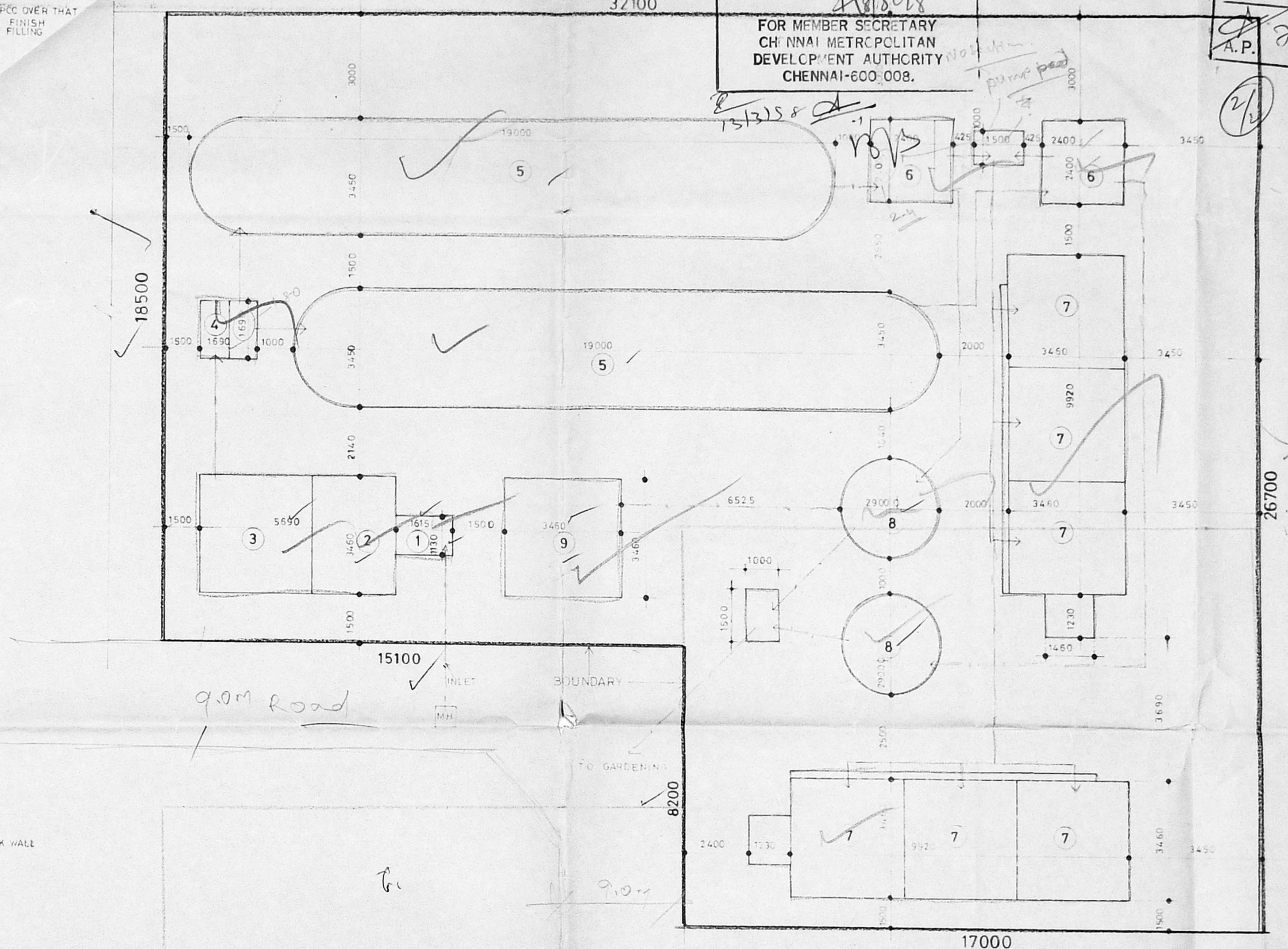
SITE PLAN
