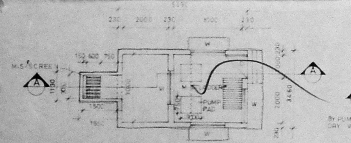
PLAN OF SCREEN, WETWELL & DRYWELL (1, 2, 3)
